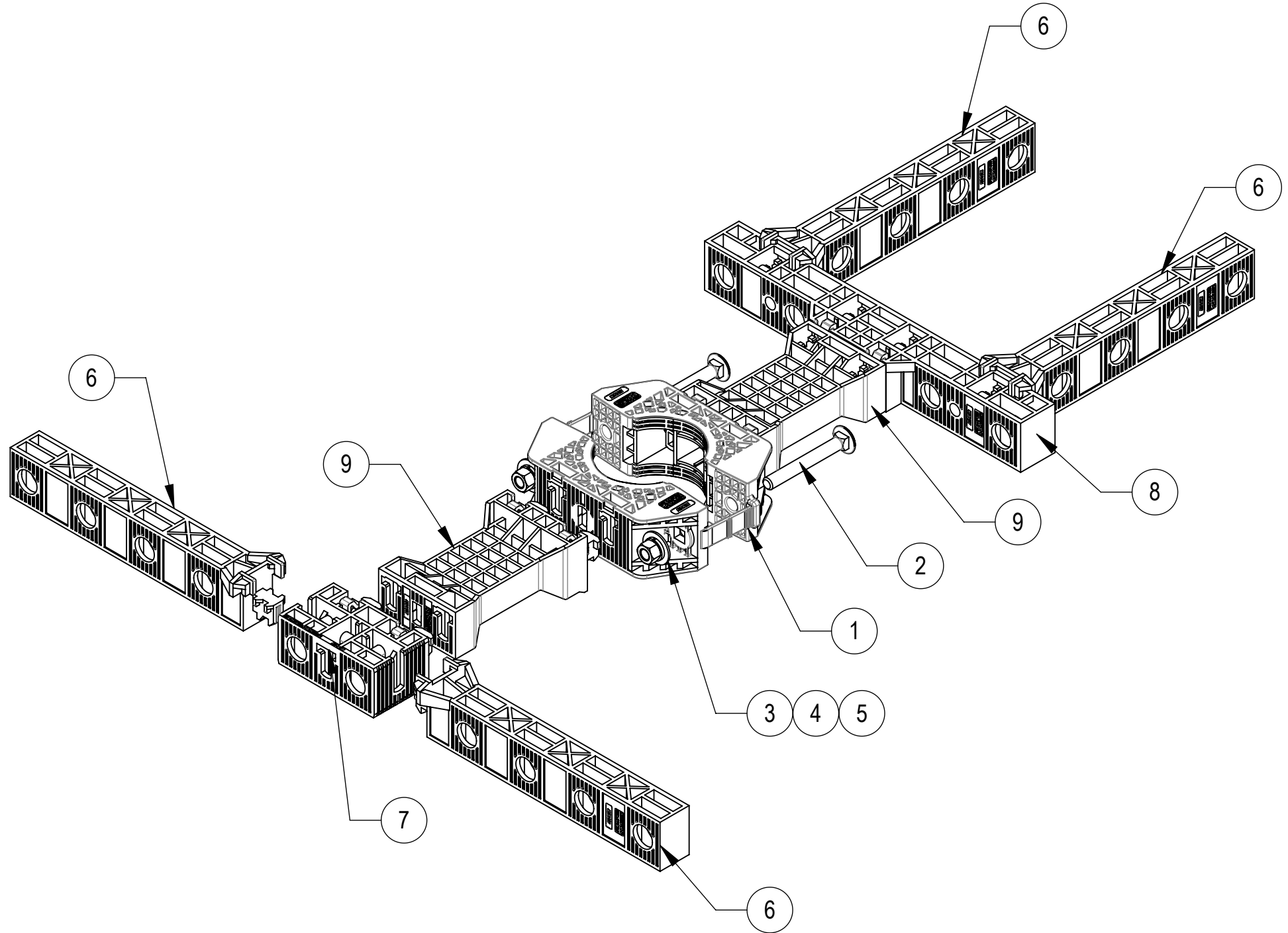
INSTALLATION ASSEMBLY
