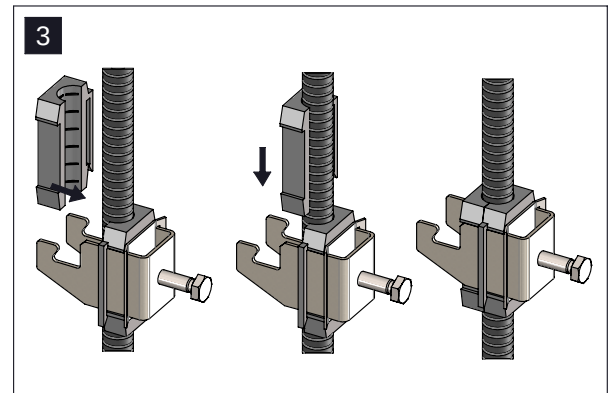
Step 3: Reinsert the plastic block into the clamp to securely fix the cable in place. Repeat the steps 1-2-3 for each cable.
