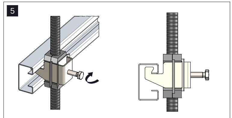
Step 5: Tighten the self-locking screw to 5 N·m torque to complete the installation.
