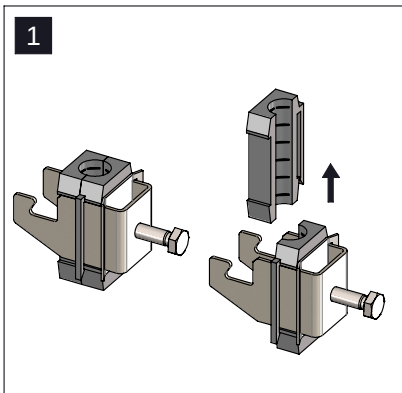
Step 1: Remove the plastic block from the cable clamp.
