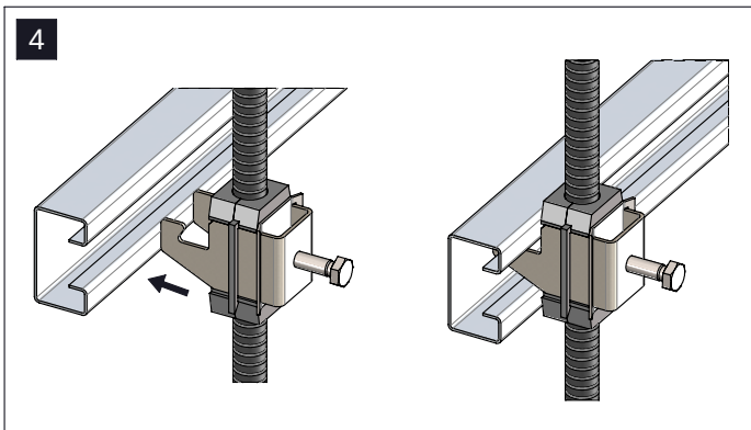
Step 4: Slide the assembled cable clamp into the rail channel and ensure it is fully seated.
