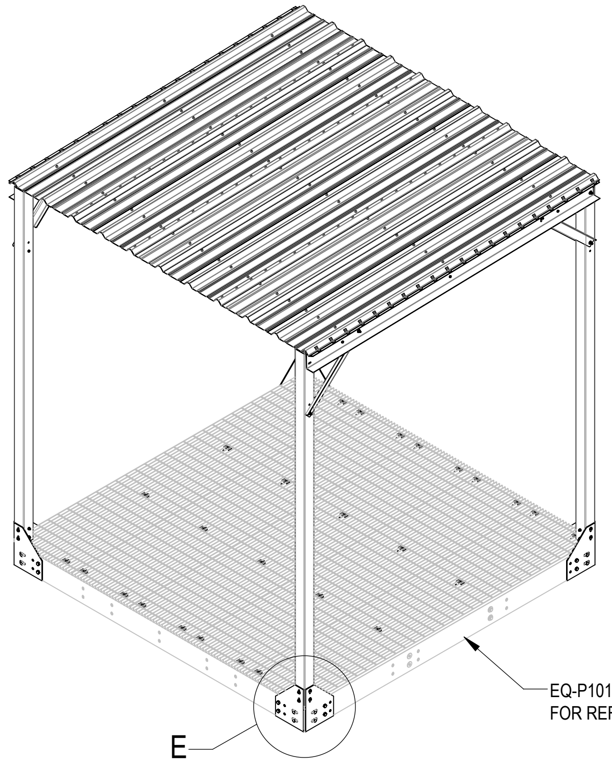
ATTACHED TO EQ-P1010-B VIEW
